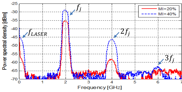
Fig. 6 16-QAM optical spectrum at the output of a single ONU, for subcarrier frequency equal to 2 GHz, m_{index} = 0.2 or 0.4 . The frequency axis is set so that f=0 corresponds to the CW laser central frequency.
