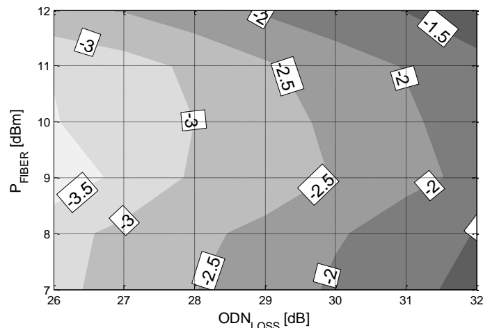
Fig. 11 BER vs ODN loss vs P_{FIBER}
