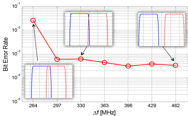
Fig. 10 Effect of frequency spacing among sub-carriers (experimental results). The insets shows for clarity the resulting spectrum (simulative results).
