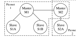
Fig. 12. Logical topology for the scenario based on Bluetooth communications, comprising two piconets.
