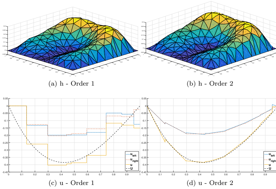
FIGURE 5.3. Solutions for benchmark problem 1 - Fracture 1
