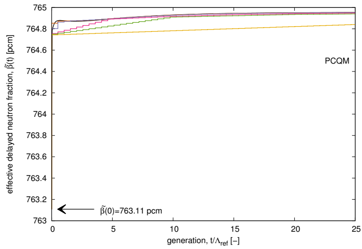
Figure 9: Time-dependent behaviour of the effective delayed neutron fraction for the compensated transient ( \Lambda_{ref} = 1.94724 \cdot 10^{-5} s). 24
