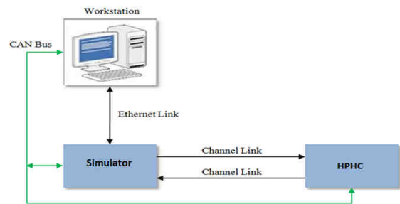
Figure 13: Test Environment
