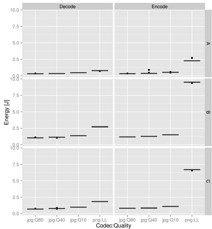
Fig. 1. Energy consumption by process, codec, and quality setting
