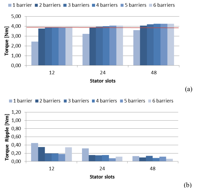
Fig. 5. Average torque (a) and standard deviation of torque ripple (b) at rated current (a) and rated speed (5000rpm) (b).
