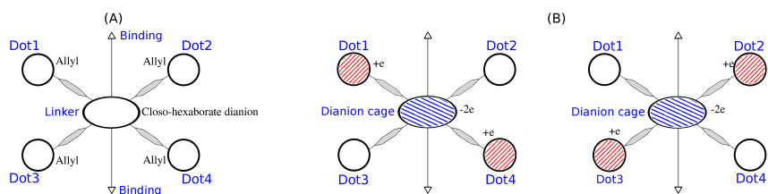
Fig. 8. The mixed-valence zwitterion: (A) structure and (B) state encoding.
