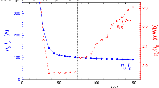
Fig. 2. Peak current in a coil n_s I_p , and resulting peak flux per turn \phi_p/n_s corresponding to the rotating peak induction B_p=1.5 T.
