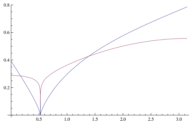
Figure 2. The parameters \omega (blue) and \lambda (red) as function of \varphi for the \mathcal{N} = 3 vacuum. The gauge group is SO(8) for \varphi < \pi/6 and SO(1, 7) for \varphi > \pi/6 . At the point \varphi = \pi/6 where \lambda vanishes, the gauge group degenerates to ISO(7) .
