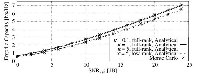
Fig. 2. Exact analysis vs. Monte Carlo simulation: Ergodic capacity vs. SNR for different values of the Rician factor and rank of LoS component.
