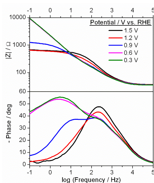
Fig. 5. Bode plots of the EIS measurements in the BV-10 electrode at different applied potentials, under AM 1.5G light illumination (100 mW cm -2 ).
