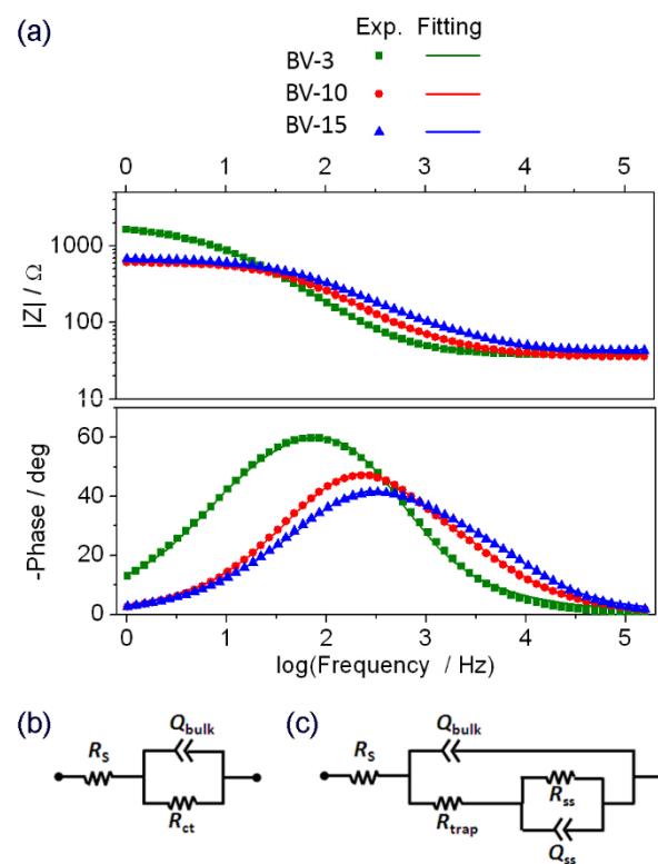
Fig. 6. Bode plots of the EIS measurements (symbols) and fitted data (lines) acquired using the BiVO 4 electrodes with different thicknesses at 0.9 V vs. Ag/AgCl (1.5 V vs. RHE) under AM 1.5G light illumination (100 mW cm -2 ). The experimental data of the BV-3 and BV-10 electrodes were fitted using the equivalent circuit (EC) depicted in (b), while the EC in (c) was employed for the BV-15 electrode.
