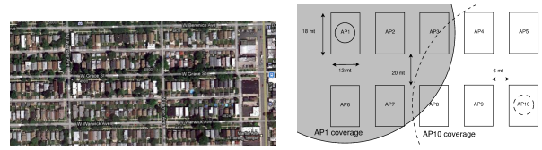
Fig. 4. Federated detached houses scenario: Google view of the area (left) and abstract representation (right). In the latter, the radio coverages of AP1 and AP10 are highlighted for the sake of example.
