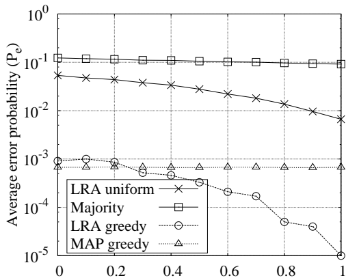
Fig. 2. Average error probability plotted versus x , for \beta = 10 and task organized in two groups of different difficulties. For the first group of tasks \pi_{t1} = 0.05, \pi_{t2} = 0.1, \pi_{t3} = 0.5 , while for the second group \pi_{t1} = 0.1, \pi_{t2} = 0.2, \pi_{t3} = 0.5 . Moreover W_1 = 30, W_2 = 120, W_3 = 150 .
