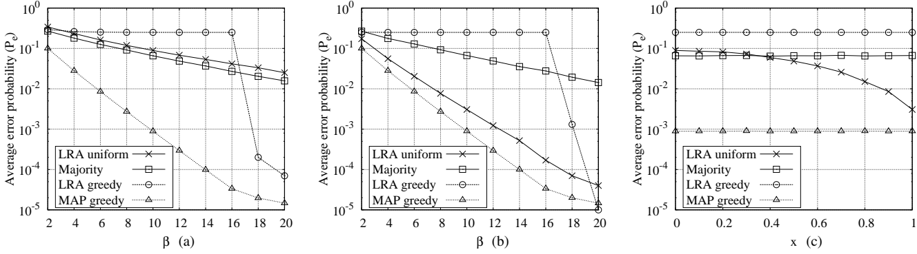
Fig. 3. Average error probability as a function of the average number of workers per task, \beta , and of the parameter x . Task organized in two groups of different difficulties. For the first group of tasks \pi_{t1} = 0.1, \pi_{t2} = 0.25, \pi_{t3} = 0.5 , while for the second group \pi_{t1} = 0.5, \pi_{t2} = 0.25, \pi_{t3} = 0.1 . Moreover W_1 = 40, W_2 = 120 and W_3 = 40 . In figures (a) and (b) we set x = 0 and x = 1 , respectively, while in figure (c) we set \beta = 10 .
