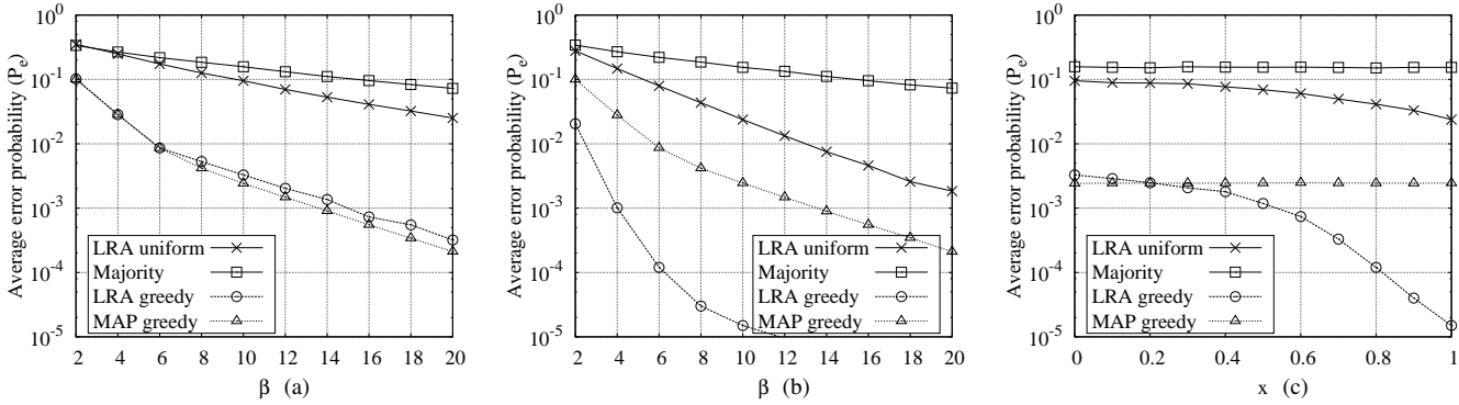
Fig. 1. Average error probability as a function of the average number of workers per task, \beta , and of the parameter x , for \pi_{t1} = 0.1, \pi_{t2} = 0.2, \pi_{t3} = 0.5 , W_1 = 30, W_2 = 120 , and W_3 = 150 . In figure (a) and (b) we set x = 0 and x = 1 , respectively, while in figure (c) we set \beta = 10 .
