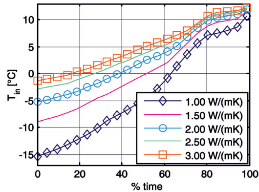
Fig. 4. Cumulate distributions of the inlet fluid temperature ( T_{in} ) for different values of the soil thermal conductivity ( \lambda^{cond} ).
