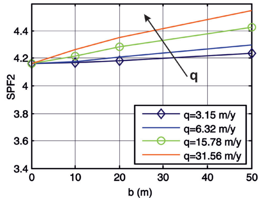
Fig. 5. SPF_2 for different values of the groundwater flow Darcy velocity ( q ) and of the aquifer saturated thickness ( b ).
