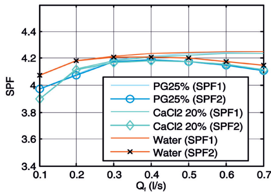
Fig. 3 – SPF 1 and SPF 2 for different heat carrier fluids and flow rates.
