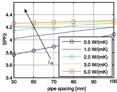
Fig. 2. GSHP Seasonal Performance Factor (SPF 2 ) for different values of the pipe spacing and of the thermal conductivity of the grout (λ g ).
