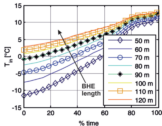
Fig. 1. Cumulate distributions of the inlet fluid temperature ( T_{in} ) for different values of the BHE length.
