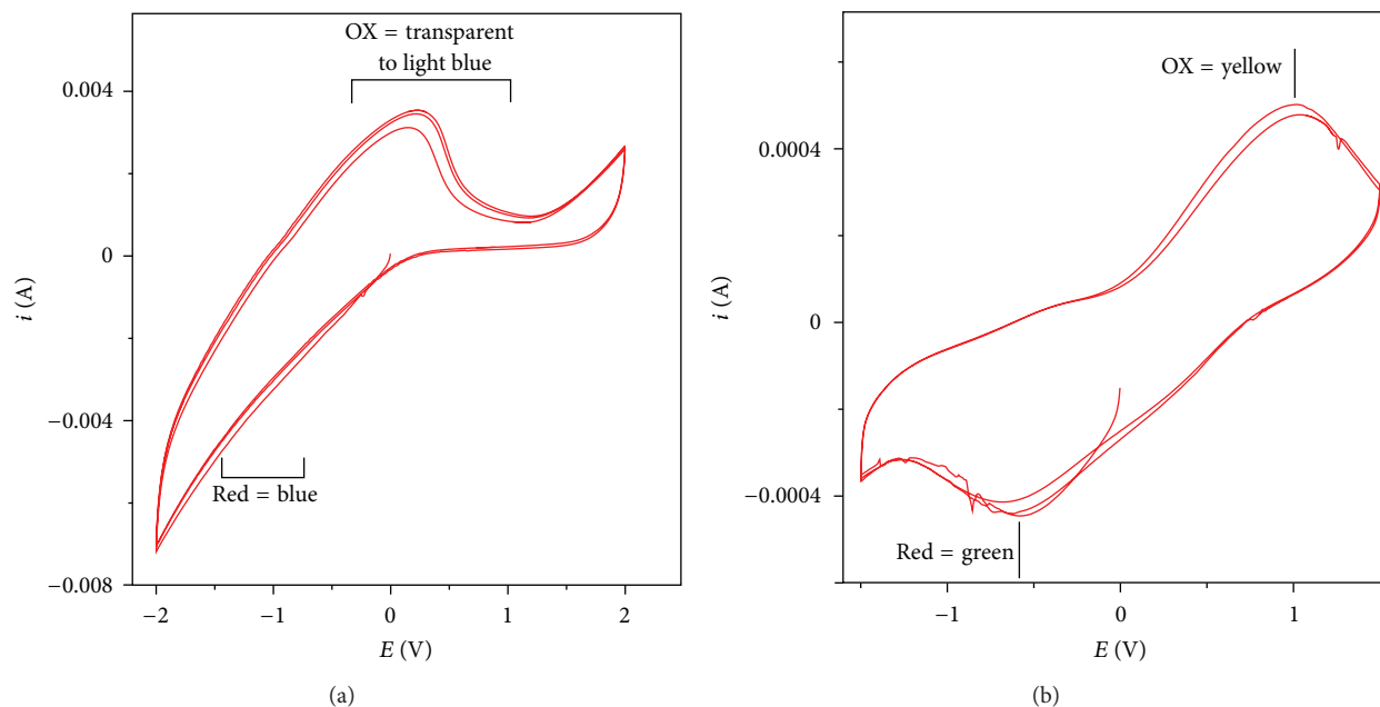
FIGURE 1: Typical CV of oxide films deposited on ITO prepared in this work. (a) \text{WO}_3 /ITO cathode in \text{LiNO}_3 0.1M aqueous solution. (b) \text{V}_2\text{O}_5 /ITO Anode in \text{LiNO}_3 0.1M ethanol solution. Electrodes configuration: ITO/Oxide film as working, Pt as counter, Sat. Ag/AgCl as reference. Scan rate 0.2 V/s. Color change is well visible by naked eye during scansion for both \text{WO}_3 and \text{V}_2\text{O}_5 . In the plots RED stands for reduced form and OX for oxidized form.
