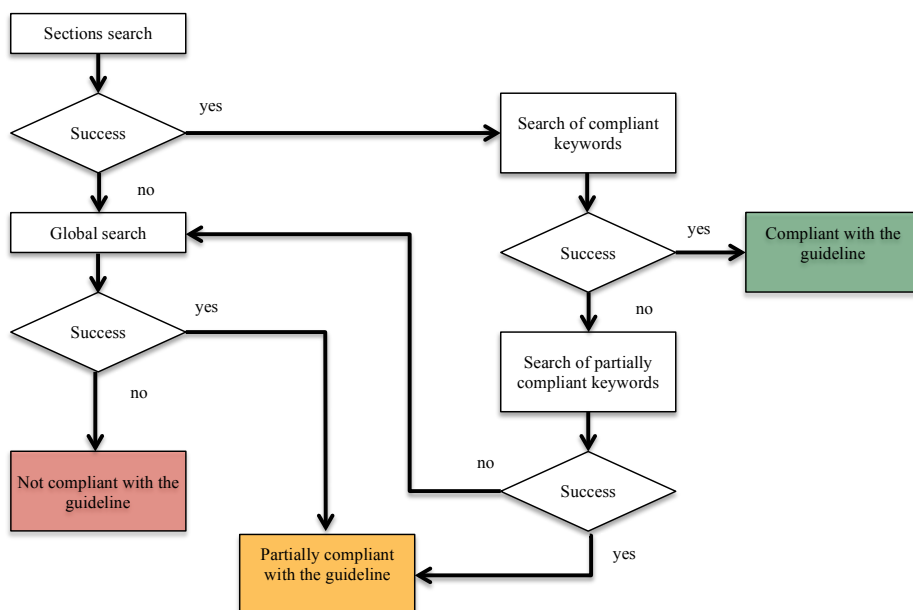
Figure 3– Parser flow
