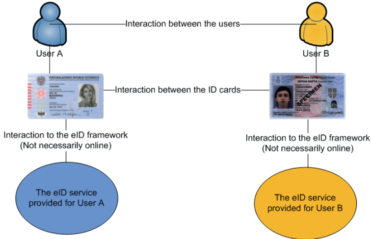
Figure 2 Peer-to-peer functionality
