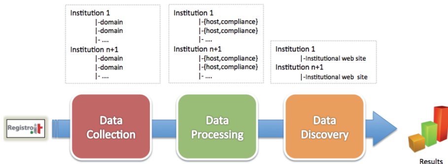
Figure 2 - SmartPA engine
