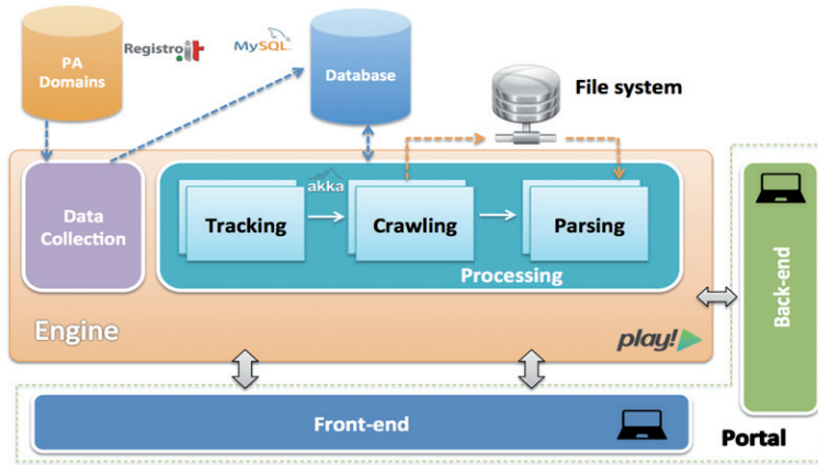
Figure 1 - SmartPA architecture
