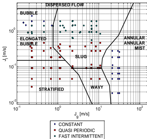
Fig. 5 Flow characterization results compared with the Mandhane’s Map flow pattern classification
