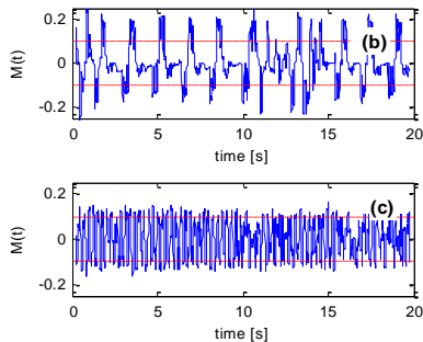
Fig. 4 M(t) time evolution at j=8 . (a) J_g=0.23 m/s - J_l=1.86 m/s, (b) J_g=2.26 m/s - J_l=0.65 m/s, (c) J_g=8.73 m/s - J_l=1.86 m/s
