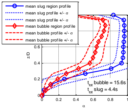
Fig. 10 Void fraction profile analysis for the “quasi periodic” flows at J_l = 0.65 \text{ m/s} - J_g = 2.26 \text{ m/s}
