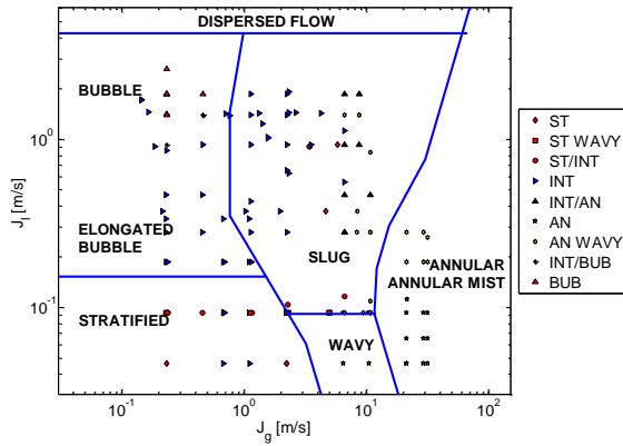
Fig. 3 Comparison between Mandhane’s Map flow patterns prediction and visual observation. Legend: ST=Stratified, INT=Intermittent, AN=Annular, BUB=Bubble. For the other symbols see paragraph 4.
