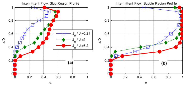
Fig. 12 “Quasi periodic” void fraction profiles dependence on the ratio J_g/J_l for slug region(a) and bubble region (b)
