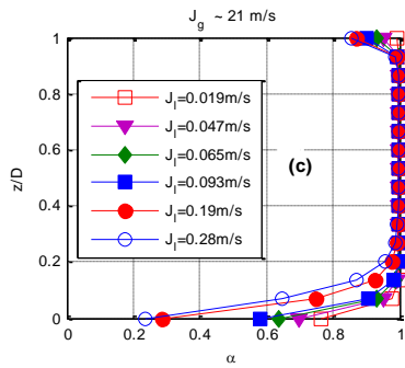
Fig. 13 Void fraction profiles at different air velocity: (a) J_g=2.33 \text{ m/s} , (b) J_g=11 \text{ m/s} , (c) J_g=21.21 \text{ m/s}
