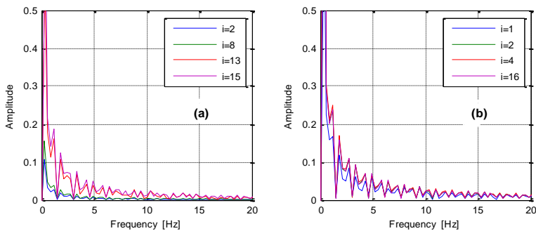
Fig. 7 Frequency spectrum at j=8 for non-intermittent flows. (a) J_g=0.23 m/s – J_l=1.86 m/s, (b) J_g=29.3 m/s – J_l=0.05 m/s
