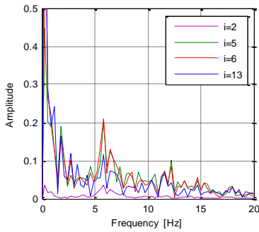
Fig. 11 Frequency spectrum at j=8 for J_l = 0.65 \text{ m/s} - J_g = 2.26 \text{ m/s}
