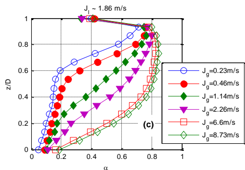
Fig. 14 Void fraction profiles at different water velocity: (a) J_t=0.09 m/s, (b) J_t=0.93 m/s, (c) J_t=1.86 m/s
