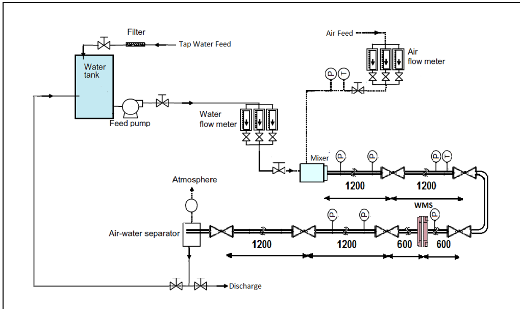
Fig. 2: Experimental facility schematic
