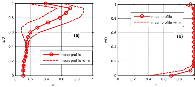
Fig. 6 Characteristic void fraction chordal profile for non-intermittent flows. (a) J_g=0.23 m/s – J_l=1.86 m/s, (b) J_g=29.3 m/s – J_l=0.05 m/s
