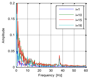
Fig. 9 Frequency spectrum at j=8 for J_l = 1.86 m/s - J_g = 8.73 m/s
