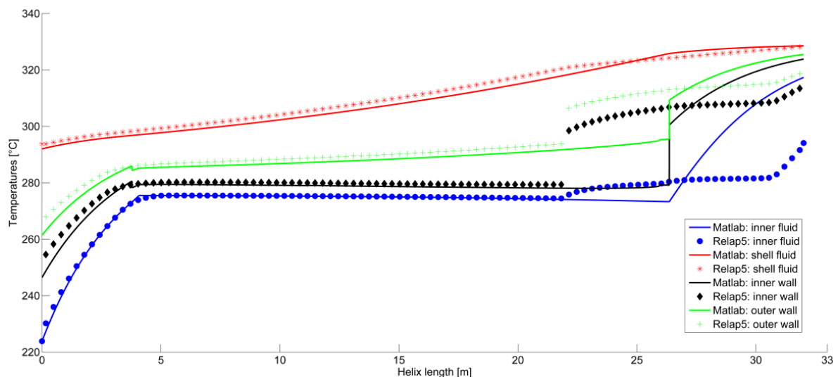
Figure 4. Temperature profiles.
