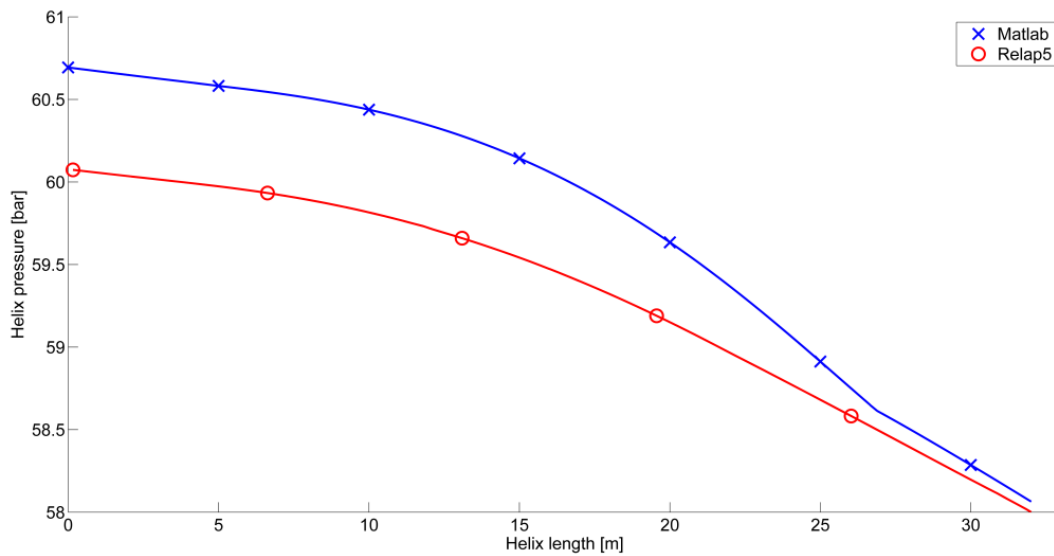
Figure 6. Internal pressure.
