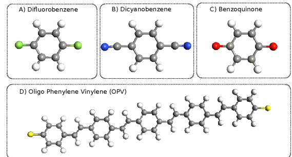
Figure 5: Different Molecules used to construct conductive channel in molecular FET. A) Benzene linked through fluorine (leftmost and rightmost atoms), B) Benzene linked through cyanide, C) Benzene linked through oxygen, D) Oligo Phenylene Vinylene in a chain of 5 molecules linked through thiol.
