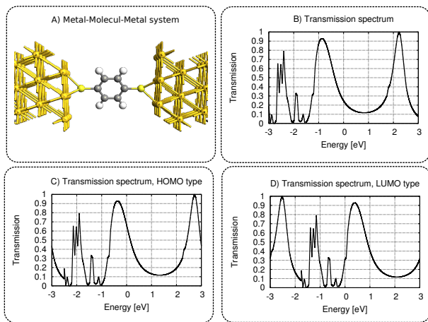
Figure 2: A) Schematic diagram of benzene molecule with thiol group sandwiched between two electrodes, B) transmission spectrum at V_{gb} = 0 , C) transmission spectrum at V_{gb} < 0 and D) transmission spectrum at V_{gb} > 0 .
