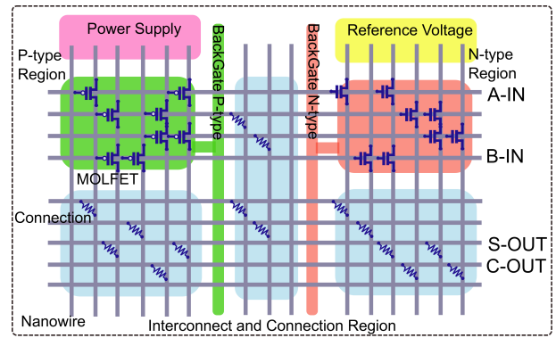
Figure 10: Crossbar architecture of Half Adder
