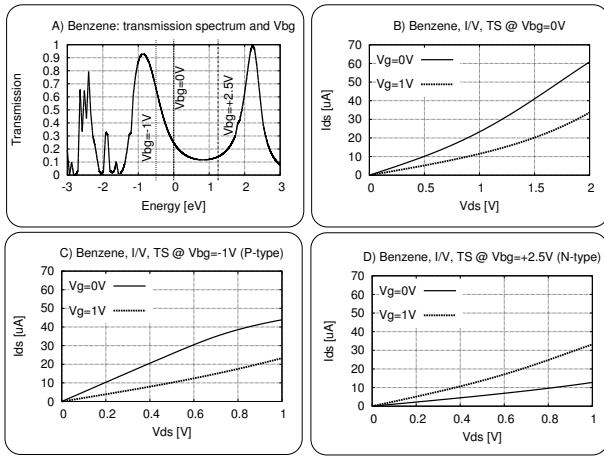
Figure 6: A) Position of E_f represented by vertical line at three different back gate volt. V_{bg} , B) I - V characteristics of benzene molecule, V_{bg} = 0V . C) I - V characteristics of benzene, V_{bg} = -1V . D) I_V characteristics of benzene, V_{bg} = 2.5V .
