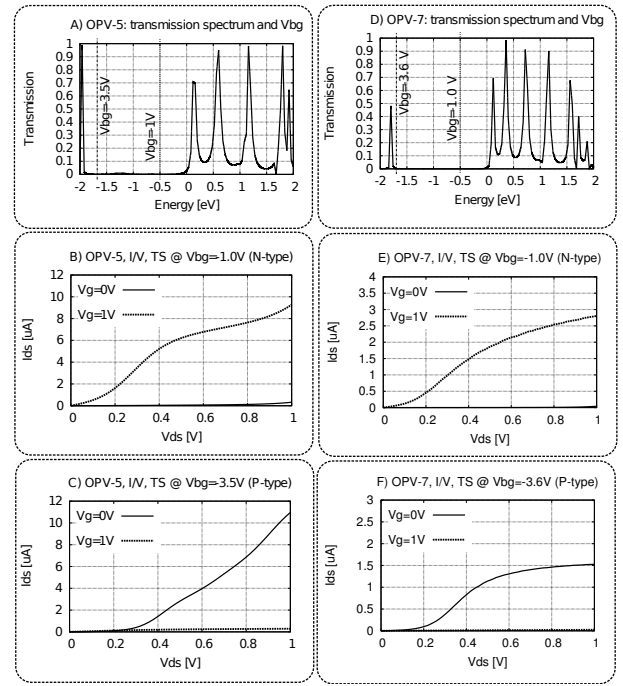
Figure 8: Transmission spectrum and I - V characteristics of OPV5 (A,B,C) and OPV7 (D,E,F) molecules. Both P-type (C,F) and N-type (B,E) obtained using different back gate voltages ( V_{bg} ) are shown in relation to their transmission spectra.
