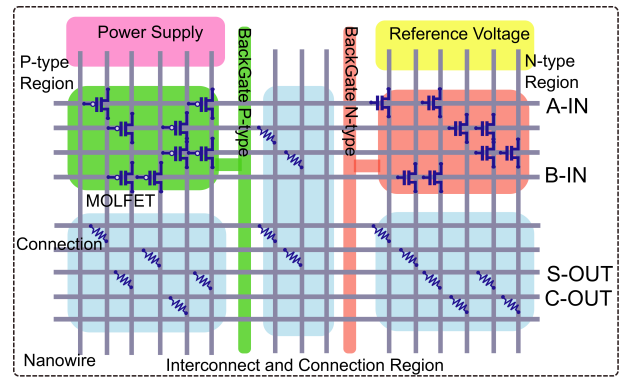
Figure 10: Crossbar architecture of Half Adder
