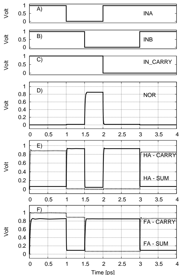
Figure 12: Output waveforms of NOR (D), HA (E) and FA (F) circuits.
