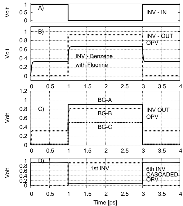
Figure 11: Output of inverter with different molecules and back gate voltages: A) inverter input. B) Inverter output for two types of molecules (OPV and benzene). C) Inverter output for OPV with three back gate voltages. BGA refers to the optimal back gate voltage: V_{bg} -P-type=-3.6V, V_{bg} -N-type=-0.9V. BGB refers to V_{bg} -P-type=-3.0V, V_{bg} -N-type=-1.5V and BGC refers to V_{bg} -P-type=-4.2V, V_{bg} -N-type=-0.3V. D) Output of six cascaded inverters.
