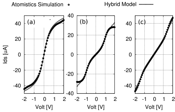
Figure 3: Comparison between the results obtained through the proposed model and the ATK simulation. I/V curves are reported for Benzene with (a) cyanide (b) oxygen and (c) Sulfur link group molecules.
