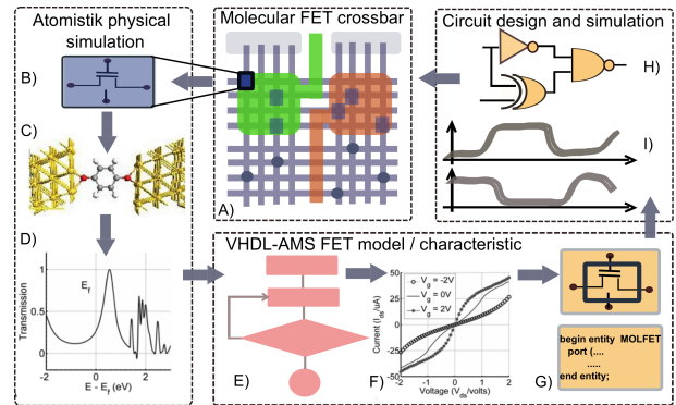
Figure 1: From device modeling to circuit simulation: A) Nanowire based crossbar architecture, B) Molecular Transistor (MT) element, C) MT Physical structure, D) MT transmission spectrum, E) Model and engine in VHDL-AMS, F) Voltage/Current (IV) characteristic, G) Modular HDL, H) Hierarchical circuits, I) Simulation output.
