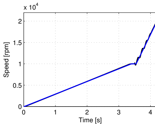
(e) Startup process, estimated speed (black) and reference speed (blue).
