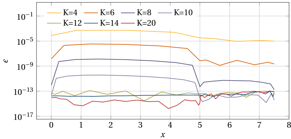
(b) P_1 approximation with c = 0.9 .
