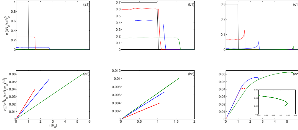
FIGURE 6.1: Ion density (1) and phase space (2) due to the explosion of a pure ion sphere composed by H + (a) and by a mixture of C + (b) and H + (c) at t = 0 (black), 24 (red), 48 (blue), 96 \sqrt{4\pi R_0^3 m_e / 3e^2 N_0} (green). The insert in figure (c2) shows a detail of the light ions multi-flow occurring at the expansion front.
