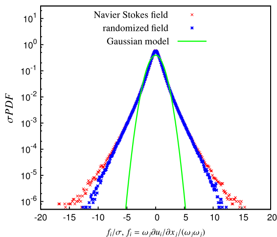
Fig. 4. PDF of the components of the vector \omega \cdot \nabla \mathbf{u} / |\omega|^2 . Comparison of the unfiltered physical field (red crosses, S = -4.81 \times 10^{-2} , K = 8.76 , variance 8.96 \times 10^{-2} ) with the Gaussian model (green line, S = 0 , K = 3 , variance 8.96 \times 10^{-2} ), and with the randomized field (blue crosses, S = -1.60 \times 10^{-2} , K = 7.46 , variance = 0.193). The pdf's are normalized on the standard deviation.
