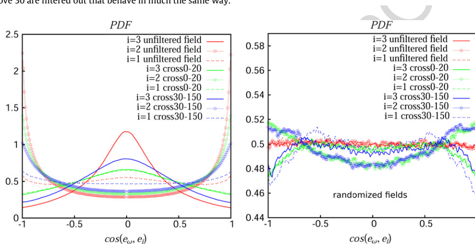
Fig. 12. PDFs of the cosine of the angle between vorticity ( \omega ), and the eigenvector, e_i , of the rate of strain tensor ( S_{ij} ). Left panel, natural NS field. Right panel, phase-randomized field. The red lines refer to the unfiltered field; the green lines refer to the case where the wave number range 0–20 is filtered out by using the high-pass cross filter; the blue lines refer to the filtering where the wave number range 30–150 is filtered out by using the band-stop cross filter.
