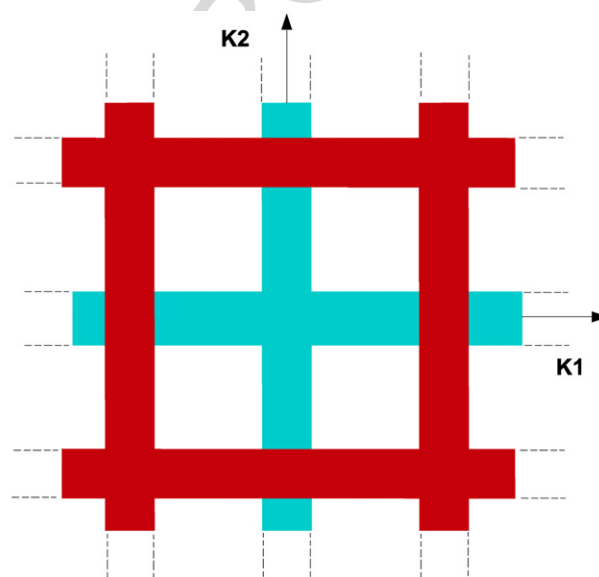
Fig. 5. Scheme of the anisotropic filter here named as CROSS filter. Blue region: high-pass filter, the wave-numbers under a certain threshold are partially removed, see Eq. (4). Red region: band-stop filter, the wave-numbers inside a range are cut, see Eqs. (5)–(7).
