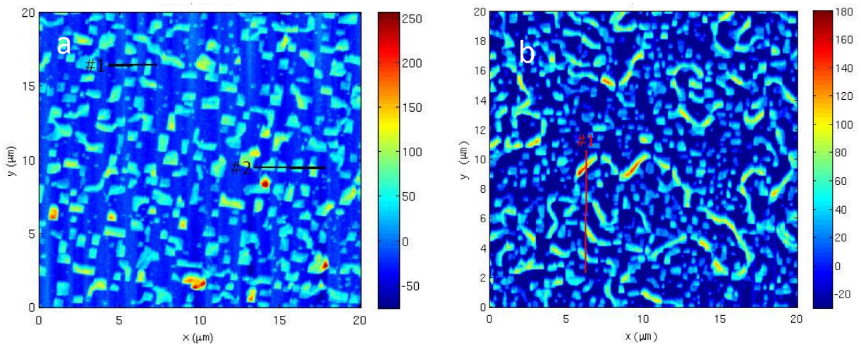
Figure 4.14: AFM images on a) sample showing marble and a stress level of 8E+08 dyne/cm 2 b) sample without marble effect and a stress level of 1.5E+09 Dyne/cm 2
