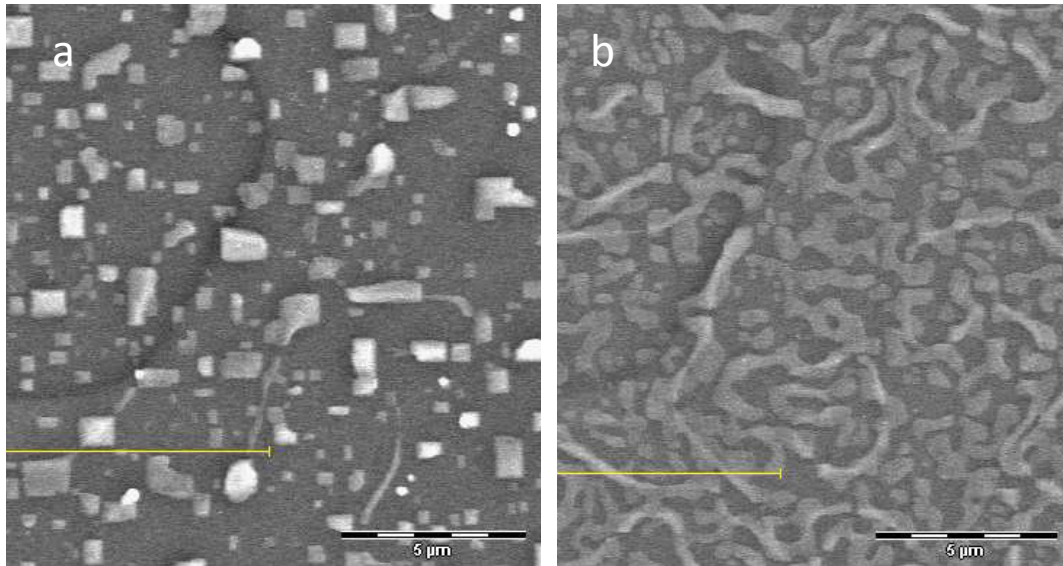
Figure 4.13: a) Interface on a sample showing marble and a stress level of 8E+08 dyne/cm 2 b) interface on a sample without marble effect and a stress level of 1.5E+09 Dyne/cm 2
