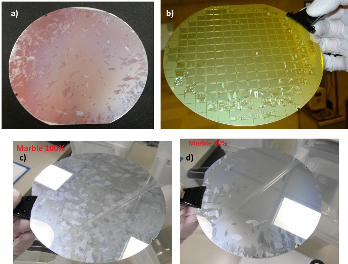
Figure 3.16 wafers with marble effect. a) Plain silicon wafer b) production wafer c) a wafer with 100% of the surface covered by marble effect d) a wafer affected by marble effect at 20%
