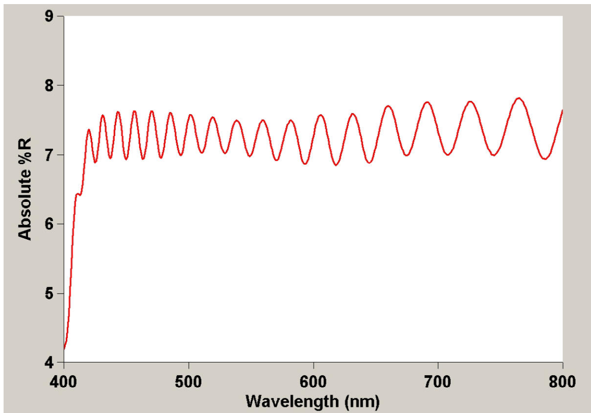
Figure 2.23: Interferences fringes
