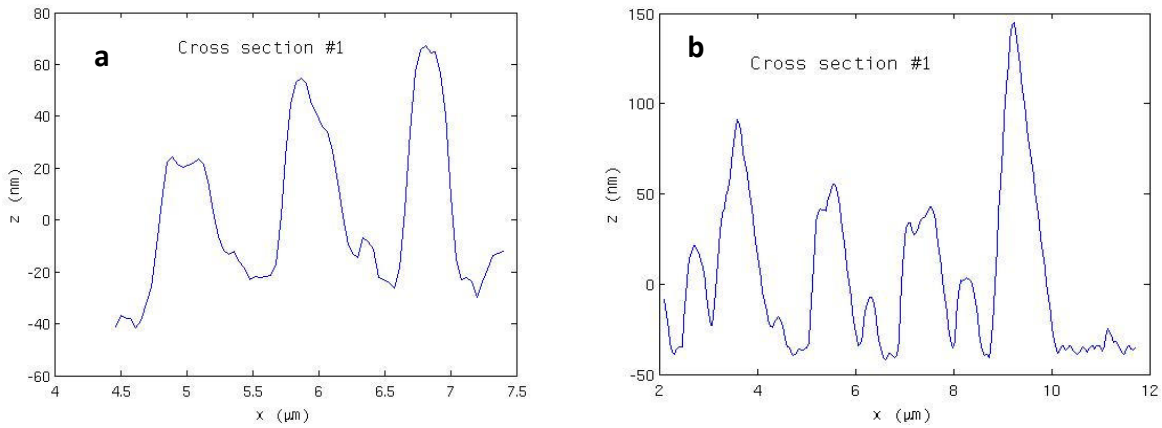
Figure 4.15: Profiles taken from AFM a) sample showing marble and a stress level of 8E+08 dyne/cm 2 b) sample without marble effect and a stress level of 1.5E+09 Dyne/cm 2
