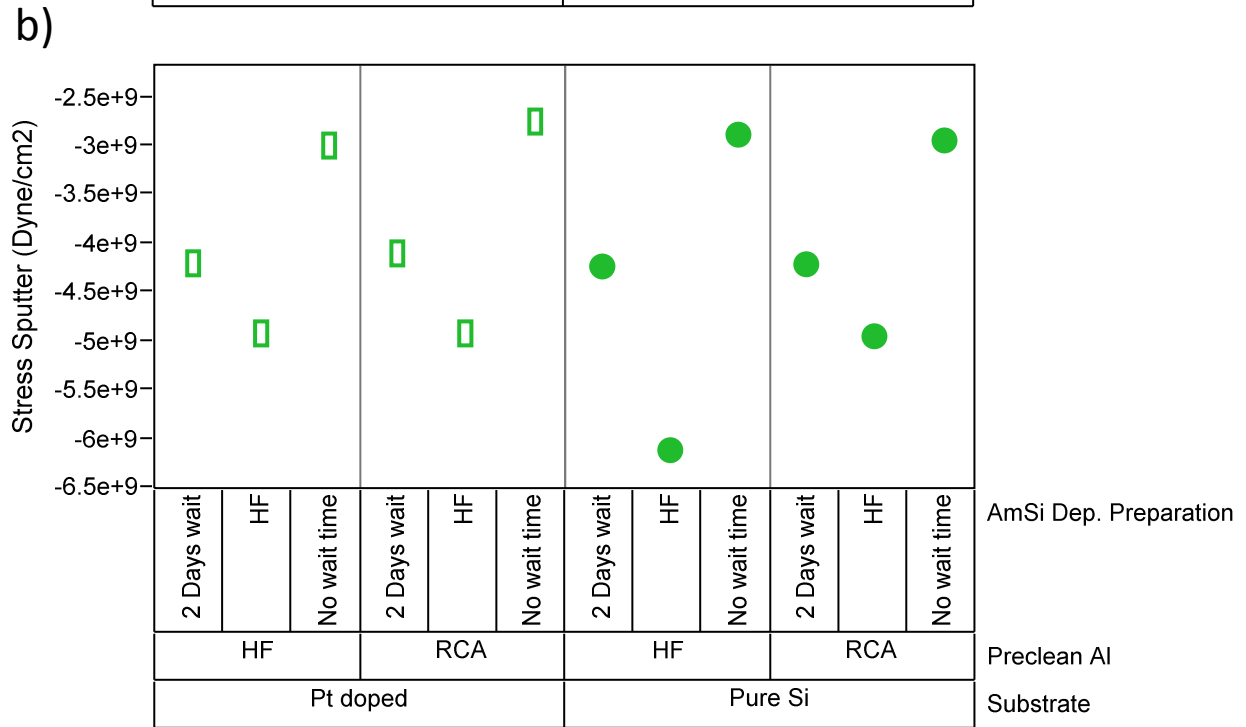
Figure 6.14. Experiment 3: a) a-Si stress after deposition b) a-Si stress after furnace sintering
