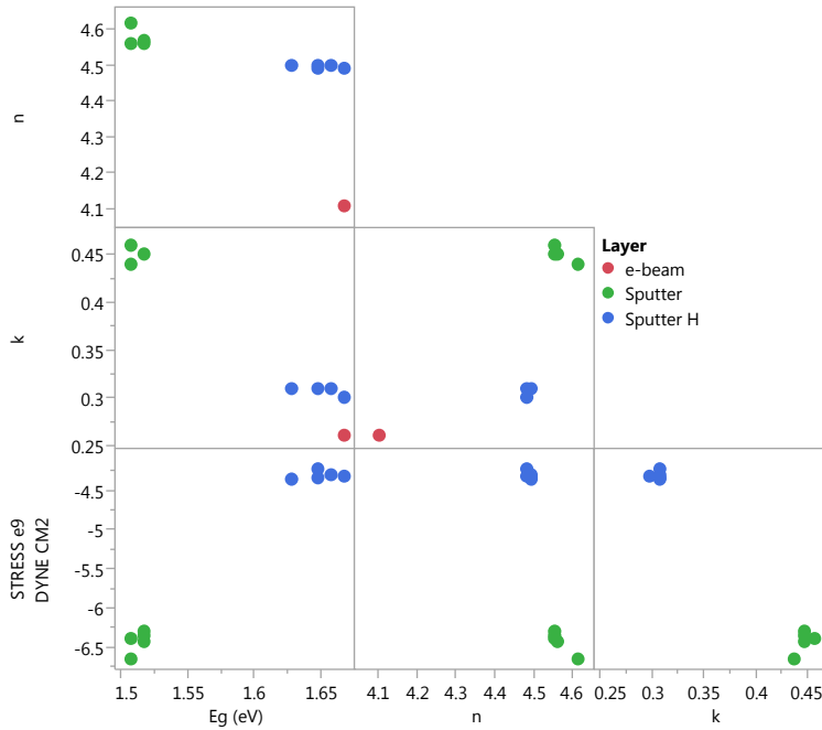
Figure 5.21: Scatterplot matrix
