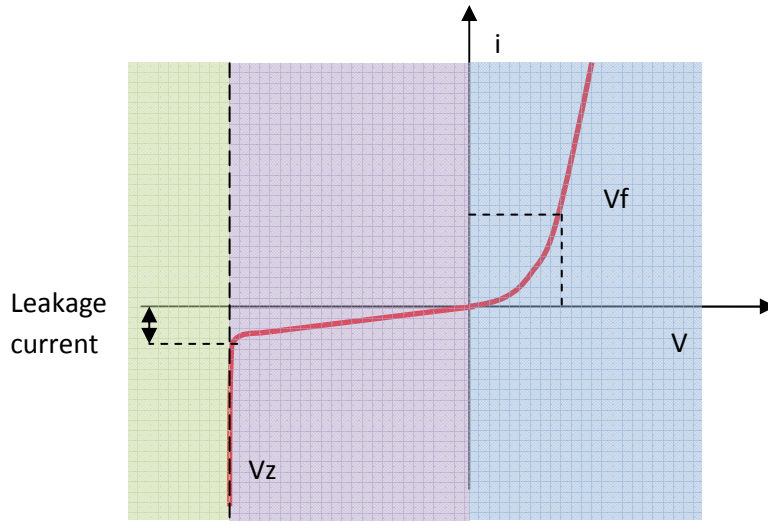
Figure 2.14 real diode
