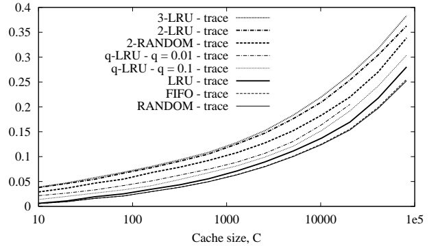
Fig. 5. Hit probability vs cache size, for various caching policies, under real trace of Youtube video requests.
