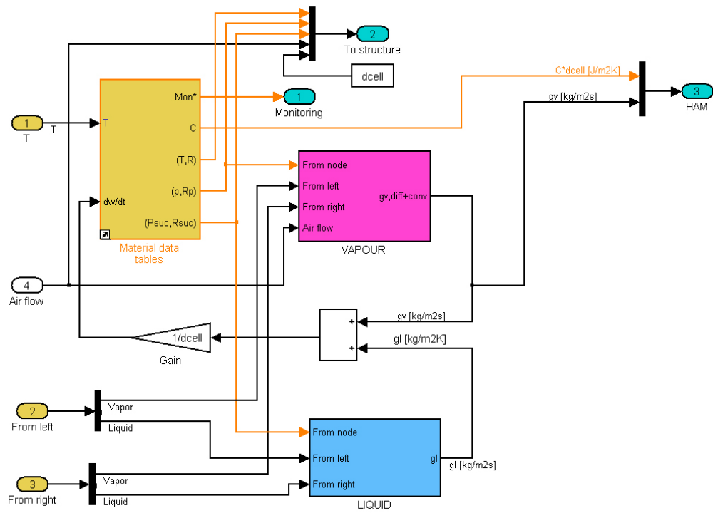
Figure 4.7: Subsystem Moisture balance .
