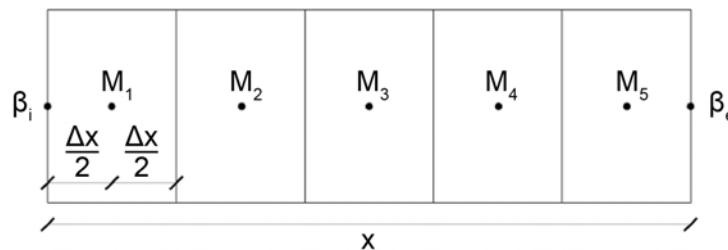
Figure 5.4: The control volumes discretization.
