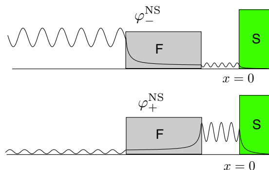
FIG. 5. (Color online) Sketch of two Majorana states, at \varepsilon = 0 , in the presence of a F barrier. Even though they do extend on the whole normal region, they are predominantly localized on one side or the other of the F domain (see text).
