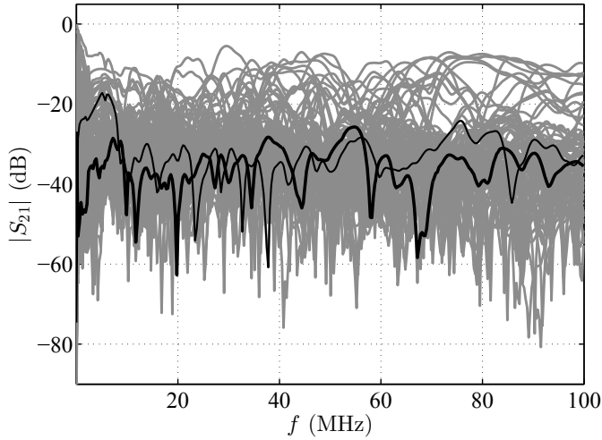
Fig. 1. Magnitude of the scattering parameter S_{21} of the power line channel of the test vehicle. The frequency range is [500\text{ Hz} \div 100\text{ MHz}] . The gray curves belong to the complete set of 106 measurements corresponding to different links and/or possible operating states of the car. The black thick lines are two example measurements in the set.
