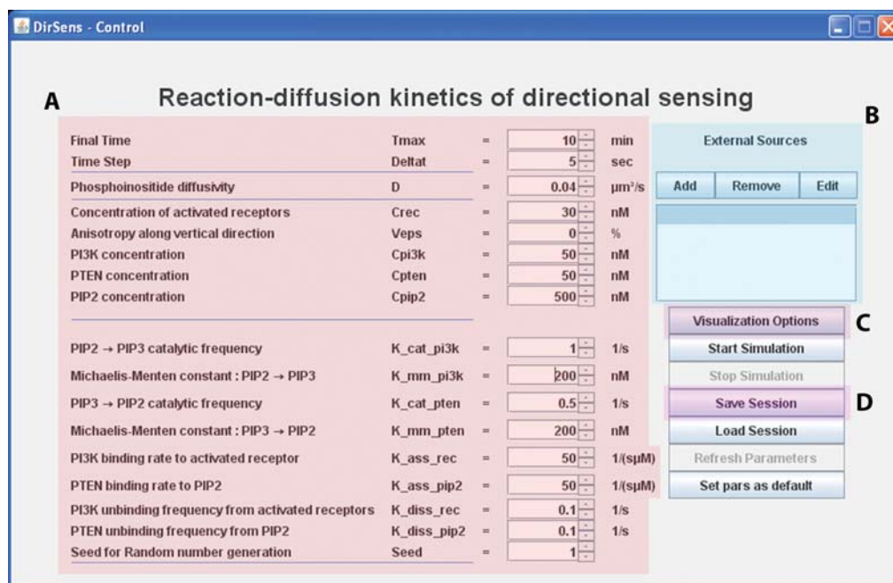
Fig. 1. The main control panel of the DirSens Simulation Environment. (A) Kinetic and physical constants are adjustable. (B) Coordinates and intensities of one or more localized chemoattractant sources can be set. (C) The user can specify the visualization in real time of different quantities, such as local or global concentration of chemical factors. (D) Simulation sessions can be saved and recalled for future analysis.
