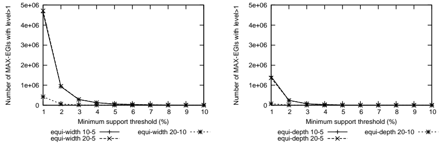
(a) Equi-width discretization.
