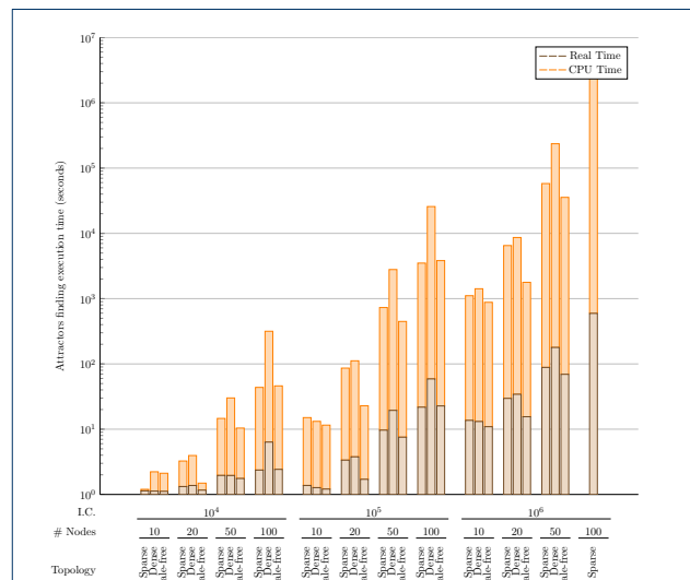
Figure 6 Time performances of the network attractors search algorithm. Experiments were performed on three different network types (Sparse, Dense, and Scale Free) with different number of nodes (10, 20, 50, and 100). For each network experiments were repeated with 10K, 100K, and 1M initial random states. Each bar represents the average of 10 experiments with the same number of random initial states; Reference Hardware: Intel(R) Core(TM) i7-2670QM CPU @ 2.20GHz ; 8GB RAM 1333MHz
