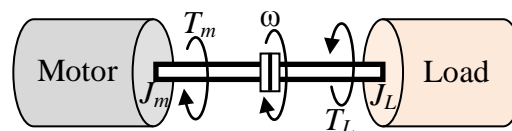
Fig. 2.5: Motor-load system
