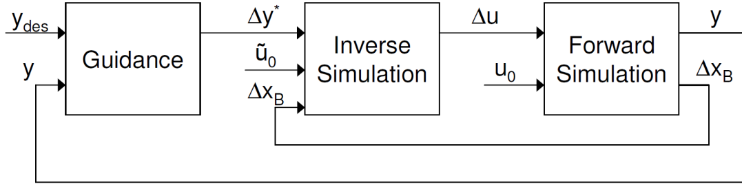
Figure 6.1: MPC-IS scheme [89].
