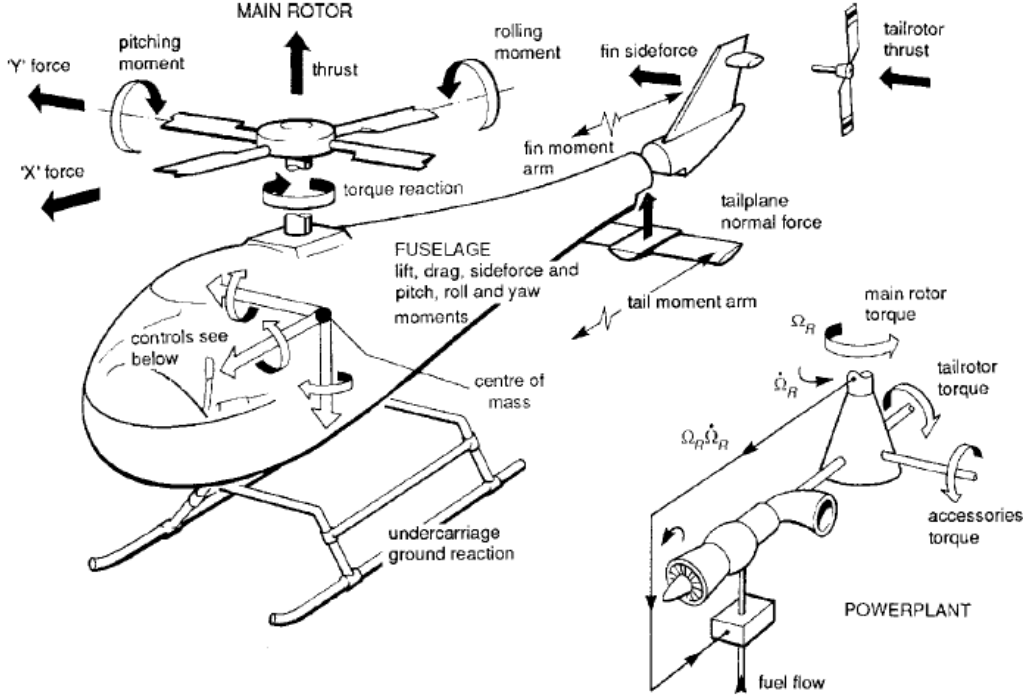
Figure 3.1: Interacting main subsystems of a helicopter [65].
