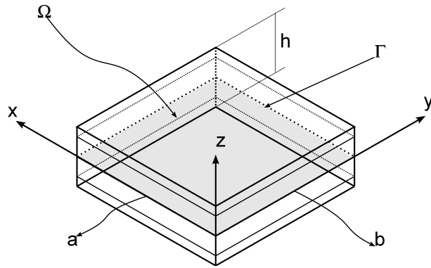
Figure 1: Plate geometry and notations. Piezoelectric configuration: actuator and sensor.
