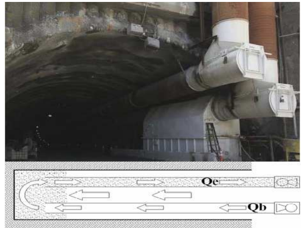
Fig. 7. The double flow ventilation system and its simplified layout used during the construction of the Caldecott Tunnel in Orinda California, fitted with an exhaust filter. Q_e should be greater than Q_b to produce an airflow toward the tunnel face. ( http://www.sfgate.com/bayarea/article/CaldecottTunnCaldecott-dig-toward-tomorrow-2309547.php#photo-1816773 )
