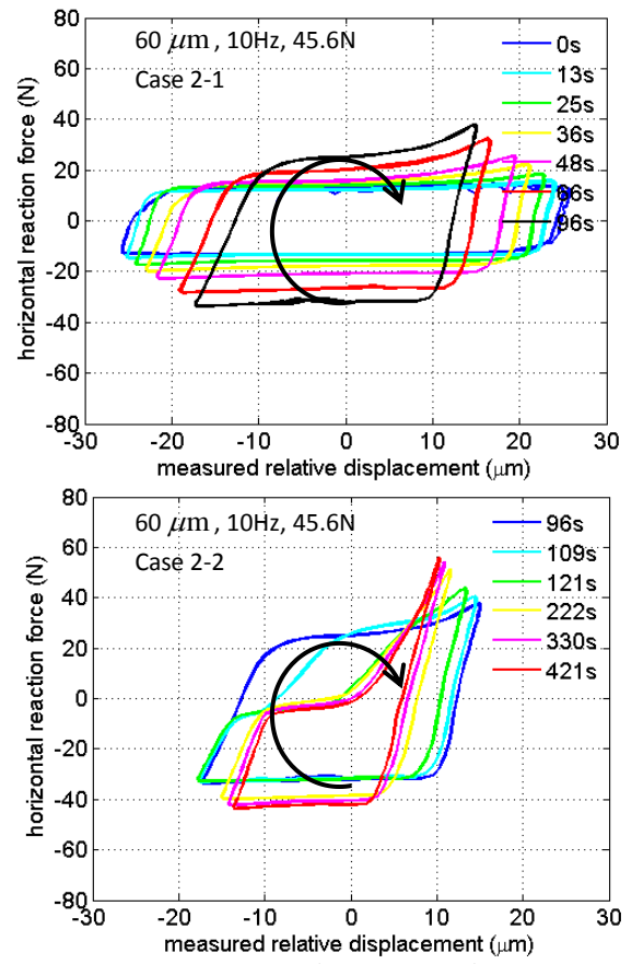
Figure 5 Hysteresis under OoP condition-Case 2
