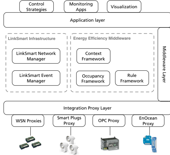
Fig. 1. Software Infrastructure
