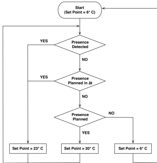
Fig. 6. HVAC Control Strategy
