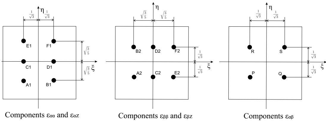
Figure 2: Tying points for the MITC9 shell element.
