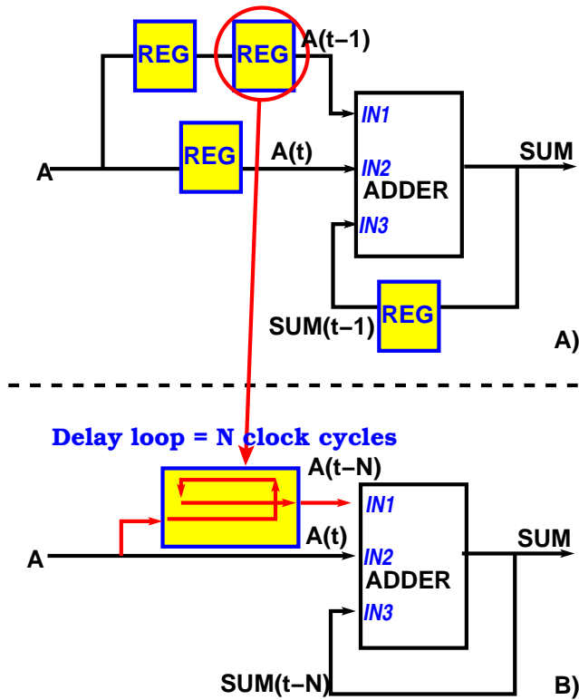
Fig. 20. Circuit example. The algorithm is SUM(t) = A(t) + A(t - 1) + SUM(t - 1) . A) CMOS implementation. B) NML implementation. An additional delay, under the form of a wire loop, is used to map the additional delay on signal A .
