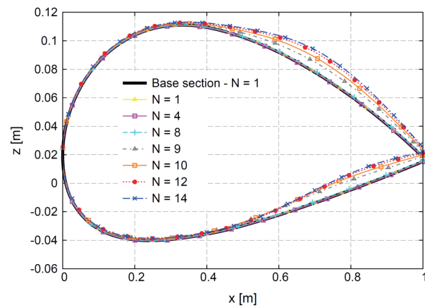
Fig. 7. Deformation of the airfoil cross-section at y=4\text{m} , computed for structural models with different accuracy. V_\infty=30\text{m/s} .
