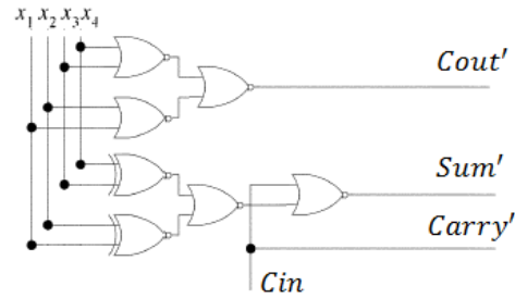
Figure 6. Gate level implementation of Design 1
