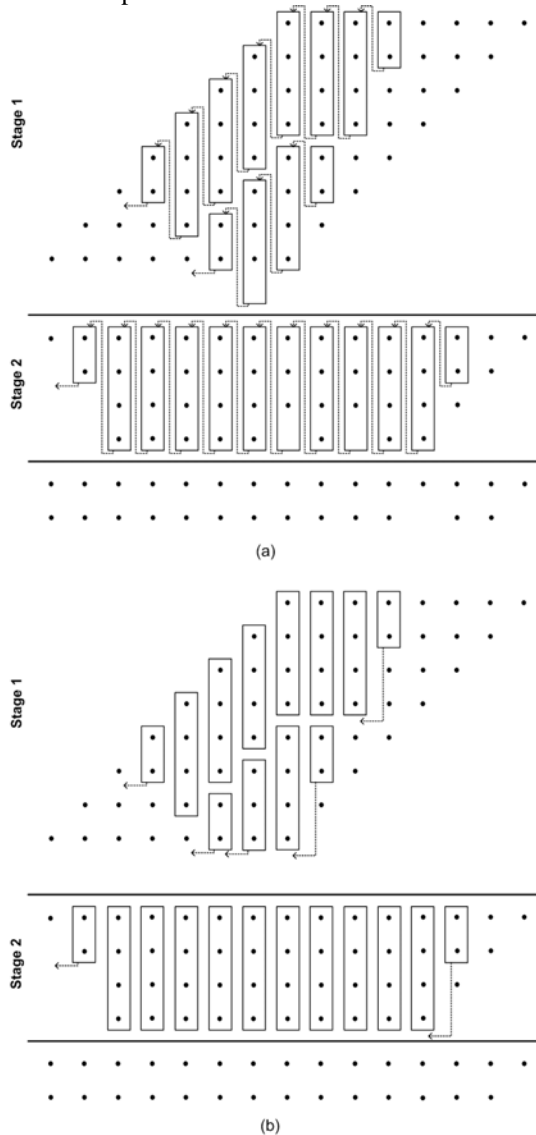
Figure 9. Reduction circuitry of an 8 \times 8 Dadda multiplier, (a) using Design 1 compressors, (b) using Design 2 compressors
