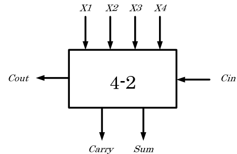
Figure 2. 4-2 compressor
