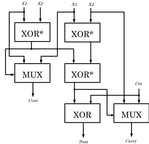
Figure 4. Optimized 4-2 compressor of [8]
