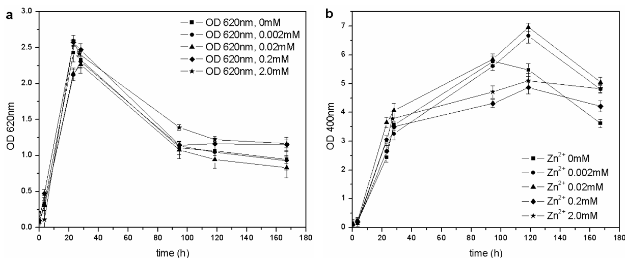
Figure 7. (a) Biomass growth in cultures supplemented with \text{ZnSO}_4 . (b) Pyoverdine production ( \text{OD}_{400} ) in cultures supplemented with \text{ZnSO}_4 .
