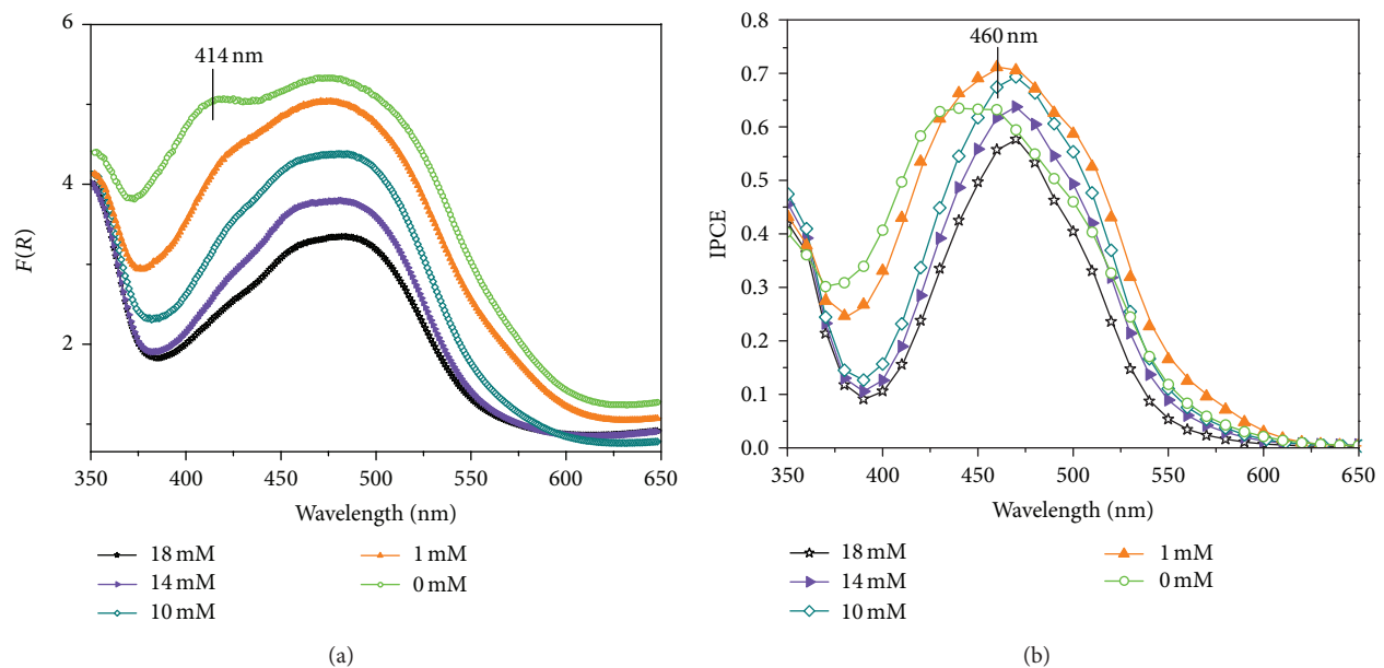
FIGURE 5: (a) UV-Visible absorbance spectra of \text{TiO}_2 photoanodes sensitized in CT1 dye for 1 hour at different CDCA concentrations. (b) IPCE action spectra of CT1-based DSCs for the same sensitization time and CDCA concentrations.
