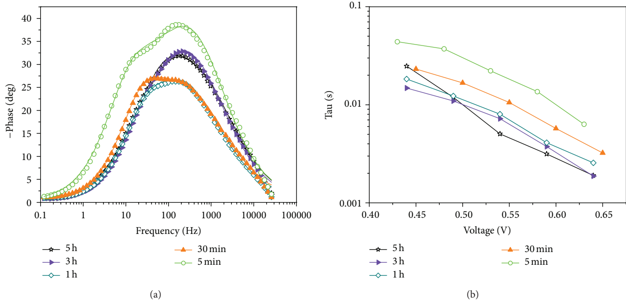
FIGURE 4: (a) Bode plots of hemi-squaraine-based solar cells for different sensitization times measured at open circuit voltage (the symbols represent the experimental data, while the continuous lines correspond to the fitting curves). (b) Electron lifetime evaluated by fitting EIS data.
