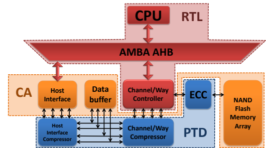
Fig. 1. Default architecture template modeled by the simulator.
