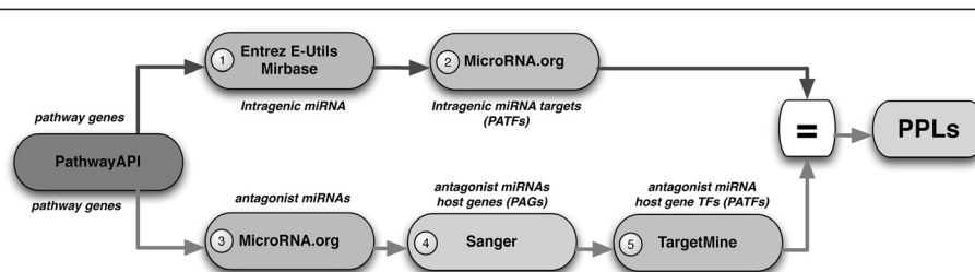
Figure 5 PPL Identification PIPELINE. Computational pipeline for the identification of pathway protection loops.
