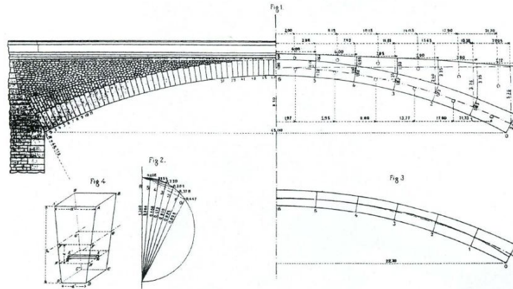
Figure 12. Geometric scheme of Mosca Bridge by Castiglano.
