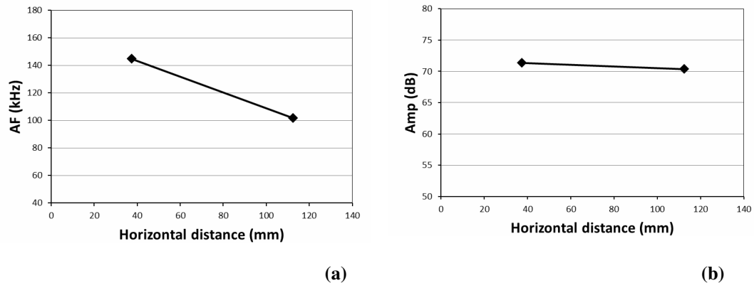
Figure 5: Specimen 1. (a) Average AF values obtained by the two sensors. (b) Average amplitude values obtained by the two sensors.
