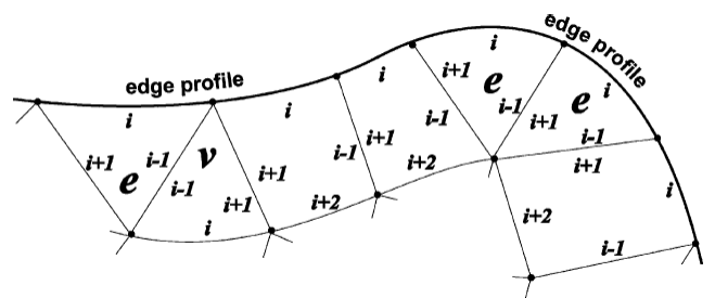
Figure 1. Edge singularity quadrilaterals and edge (e) and vertex (v) singularity triangles with local edge numbering scheme.
